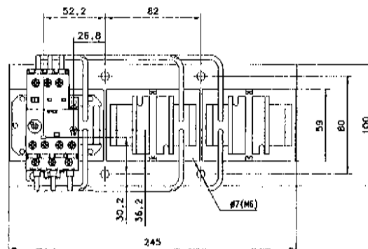
Drilling plan
