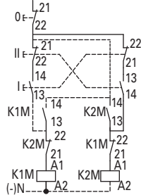
Control Circuit—40–170A
