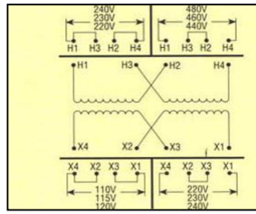
CONNECTION DIAGRAM: GROUP "P"
