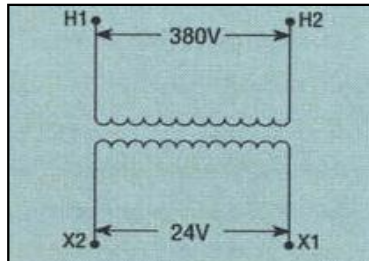
CONNECTION DIAGRAM: GROUP "G"
